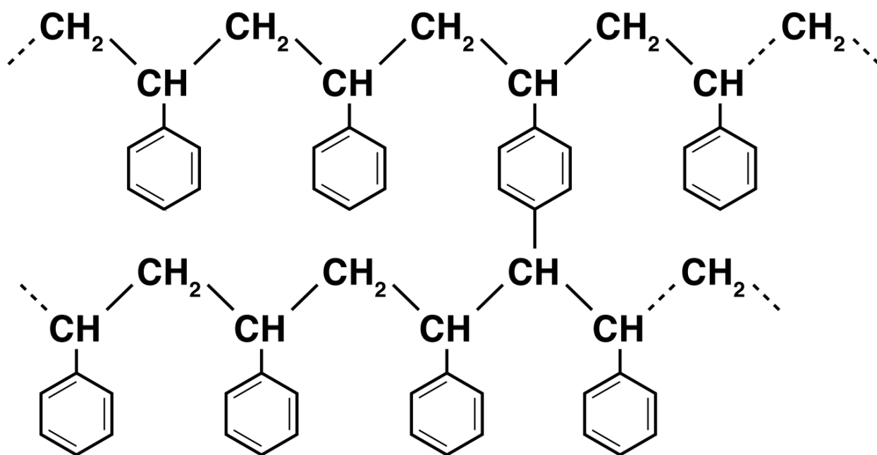
Crosslinked Polystyrene
